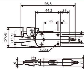
迷你夹具EM-12-C
