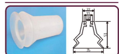
JD2-35 瓶坯吸盘
